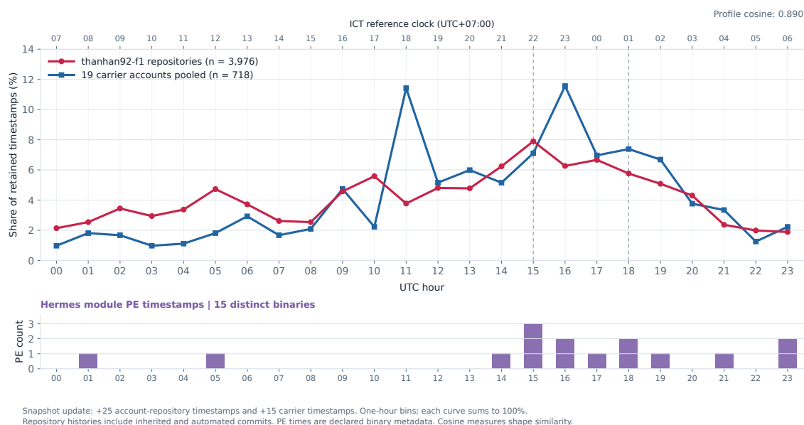
Figure 6.5 Hourly profiles compare 3,976 timestamps from the named account's repositories with 718 from nineteen carrier accounts, each normalized to its own total; cosine similarity is approximately 0.890. Fifteen module PE timestamp fields form a separate histogram. UTC+07:00 is a reference clock, not an inferred location.
