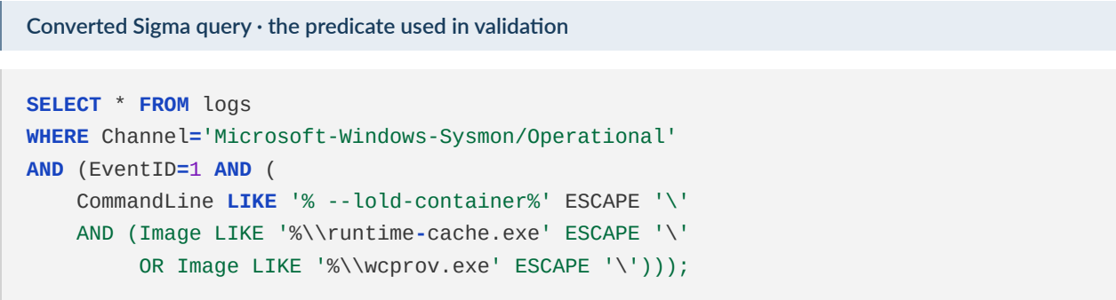
Figure 7.5 Actual SQLite query produced from the published container-child Sigma rule and executed against retained benign Sysmon records. Only whitespace is reformatted here.
